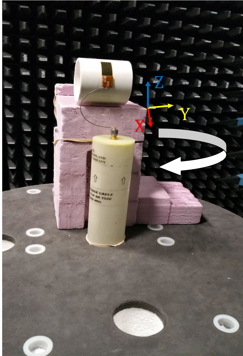
Figure 13: Outer diameter setup
