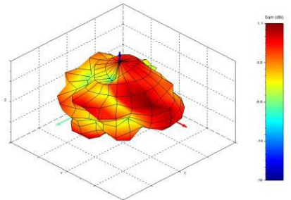
3D Radiation Pattern - Total Gain at 5900 MHz
