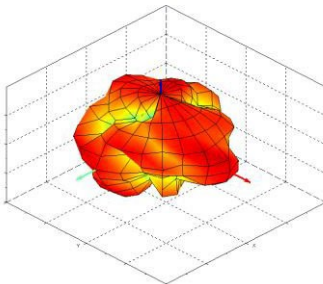
3D Radiation Pattern - Phi Polarization Gain at 5900 MHz
