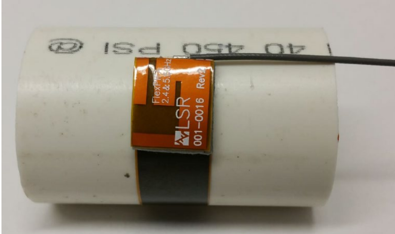
Figure 35: Convex mounted
