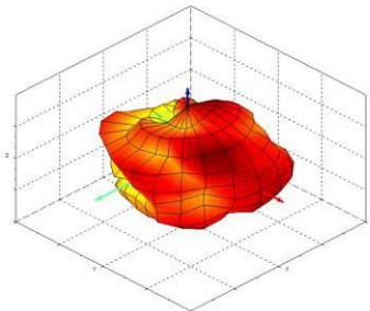
3D Radiation Pattern - Theta Polarization Gain at 5900 MHz
