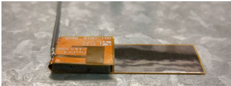
Figure 37: FlexPIFA mounted on metal
