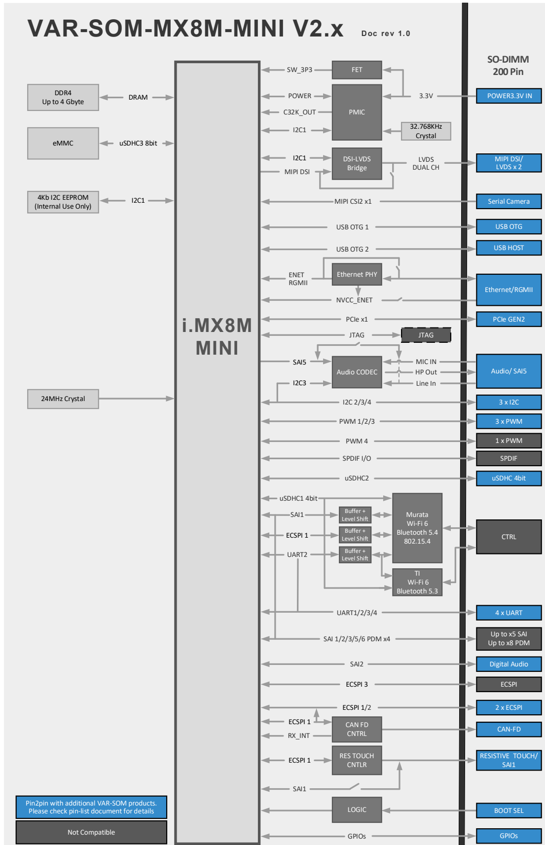
Figure 1 : VAR-SOM-MX8M-MINI Block Diagram
