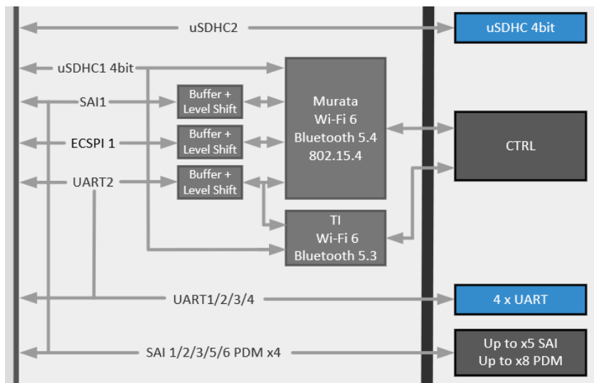
Figure 3: VAR-SOM-MX8M-MINI Wi-Fi & BT Internal Connection
